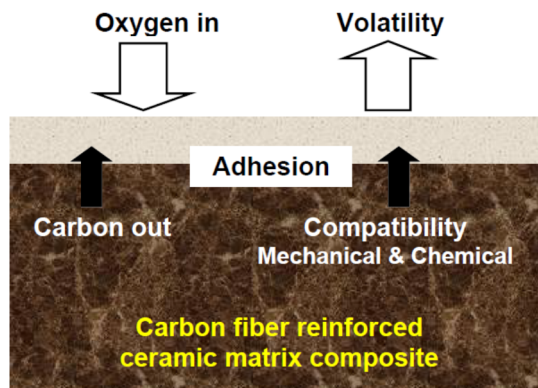
图 28 涂层的抗氧化性能的影响因素示意图 Figure 28 The influence factors of the antioxidant properties of the coatings
