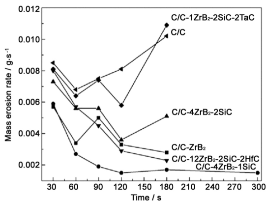
图 20 C/C-UHTC 和 C/C 复合材料在 2380 \text{ kW/m}^2 热流下的质量烧蚀率 [135] Figure 20 Mass erosion rates of C/C-UHTC and C/C composites under a 2380 \text{ kW/m}^2 heat flux [135]
