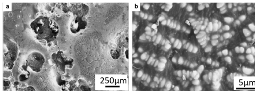
图 19 C/C-4ZrB 2 -1SiC 复合材料在 2380 \text{ kW/m}^2 热流密度下 300s 烧蚀后形貌 [135] Figure 19 Ablated surface morphology of C/C-4ZrB 2 -1SiC under a 2380 \text{ kW/m}^2 heat flux for 300 s [135]
