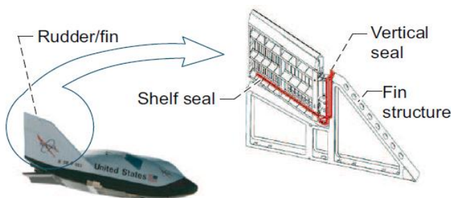
图 40 X-38 方向舵/翼面典型密封界面图解 Figure 40 Rudder / fin structure and seal locations for X-38 vehicle
