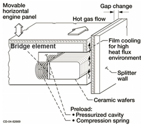
图 42 栅板式密封结构示意图 [417] Figure 42 Schematic of ceramic wafer seal structure
