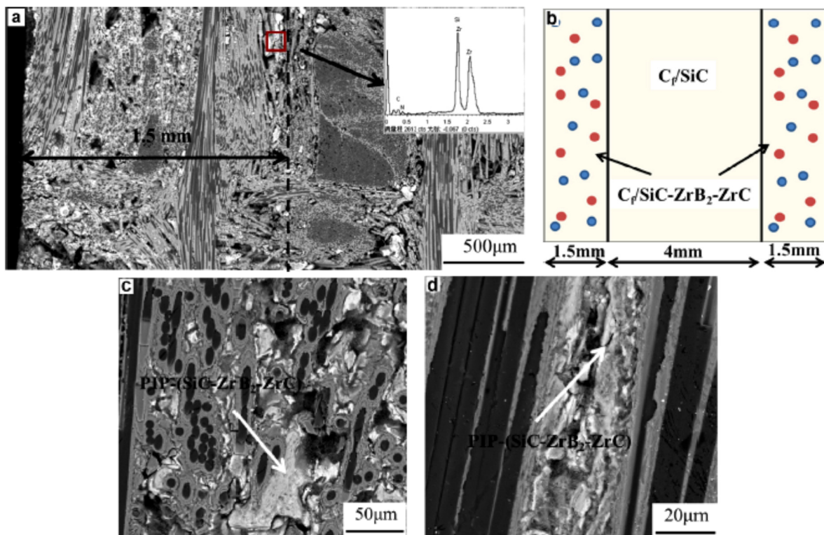
图 21 三明治结构 C f /SiC-ZrB 2 -ZrC 复合材料背散射 SEM 形貌及结构示意图: (a) 截面低倍形貌; (b) 结构示意图; (c,d) 纤维束间和层间基体分布 [119] 。(c, d) 中箭头所指为 PIP-(SiC-ZrB 2 -ZrC) 基体 Figure 21 Backscattered electron images and schematic of the sandwich-structured composites: (a) low magnification of the cross-section; (b) schematic of the composite; (c,d) higher magnifications of the region in and between bundles of the C f /SiC-ZrB 2 -ZrC composites, respectively [119] . Allows in (c) and (d) indicate the PIP-(SiC-ZrB 2 -ZrC) matrix.
