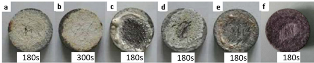
图 18 不同组成的 C/C-UHTC 复合材料在热流密度 2380 \text{ kW/m}^2 下烧蚀 180 s 或 300 s 后的表面形貌 [135] Figure 18 The surface morphologies of different C/C-UHTC composites after being ablated for 180 s or 300 s under a 2380 \text{ kW/m}^2 heat flux [135] (a) C/C-ZrB 2 ; (b) C/C-4ZrB 2 -1SiC; (c) C/C-1ZrB 2 -2SiC; (d) C/C-2SiC-1ZrB 2 -2HfC, (e) C/C-2SiC-1ZrB 2 -2TaC; (f) C/C
