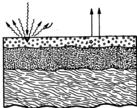
图 32 一种双层功能热控涂层 Figure 32 A double-layer functional thermal coating
