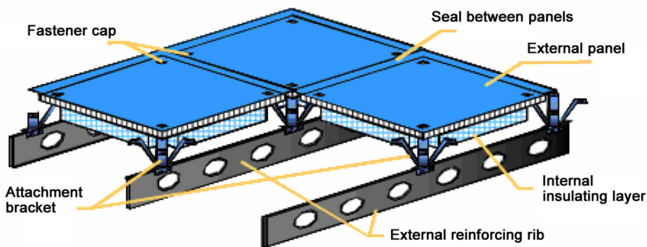
图 6 金属隔热盖板结构示意图 Figure 6 Illustration of the structural layout of the metallic thermal protection shingle
