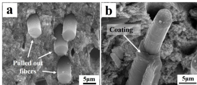
图 9 ZrB 2 -SiC-C f 复合材料的断口形貌: (a) 未涂层碳纤维; (b) 碳涂层的碳纤维 [90] Figure 9 SEM images of the fracture surface of ZrB 2 -SiC-C f composites: [90] (a) carbon fibers without coating; (b) carbon coated carbon fibers
